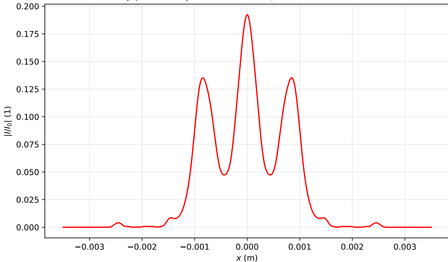
Intensity profile I(x, y = 0, z = 2.149)/I_0 , P_{in}=7.0P_{cr} , artificial time
